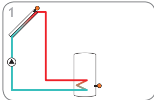
1 Standard solar system with 1 store (page 9)
