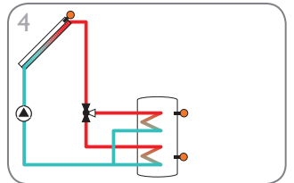
4 Solar system with 1 store and 3-port valve for store loading in layers (page 15)
