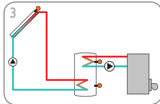
3 Solar system with 1 store and afterheating (page 13)
