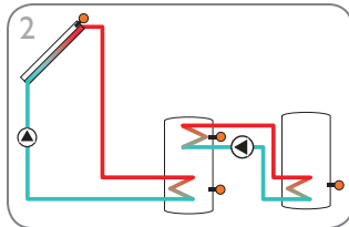
2 Solar system with 2 stores and heat exchange (page 11)
